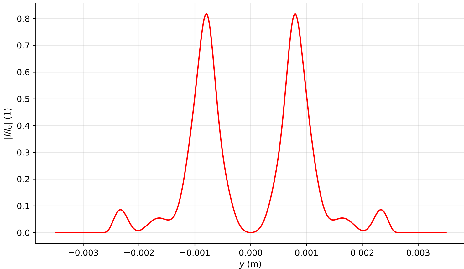
Intensity profile I(x = 0, y, z = 3.901)/I_0 , P_{in}=5.0P_{cr} , artificial time
